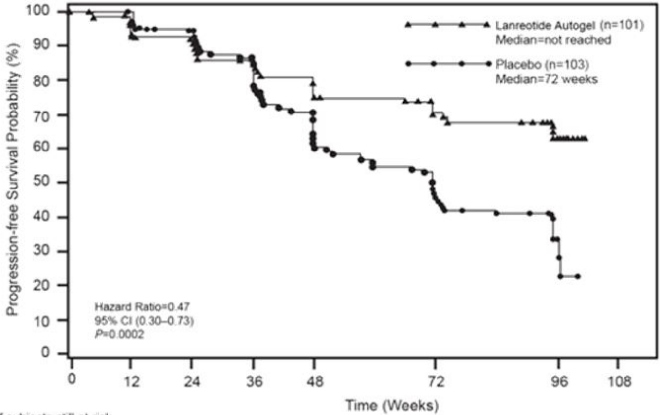
Figure 1: Kaplan-Meier Progression Free Survival Curves
