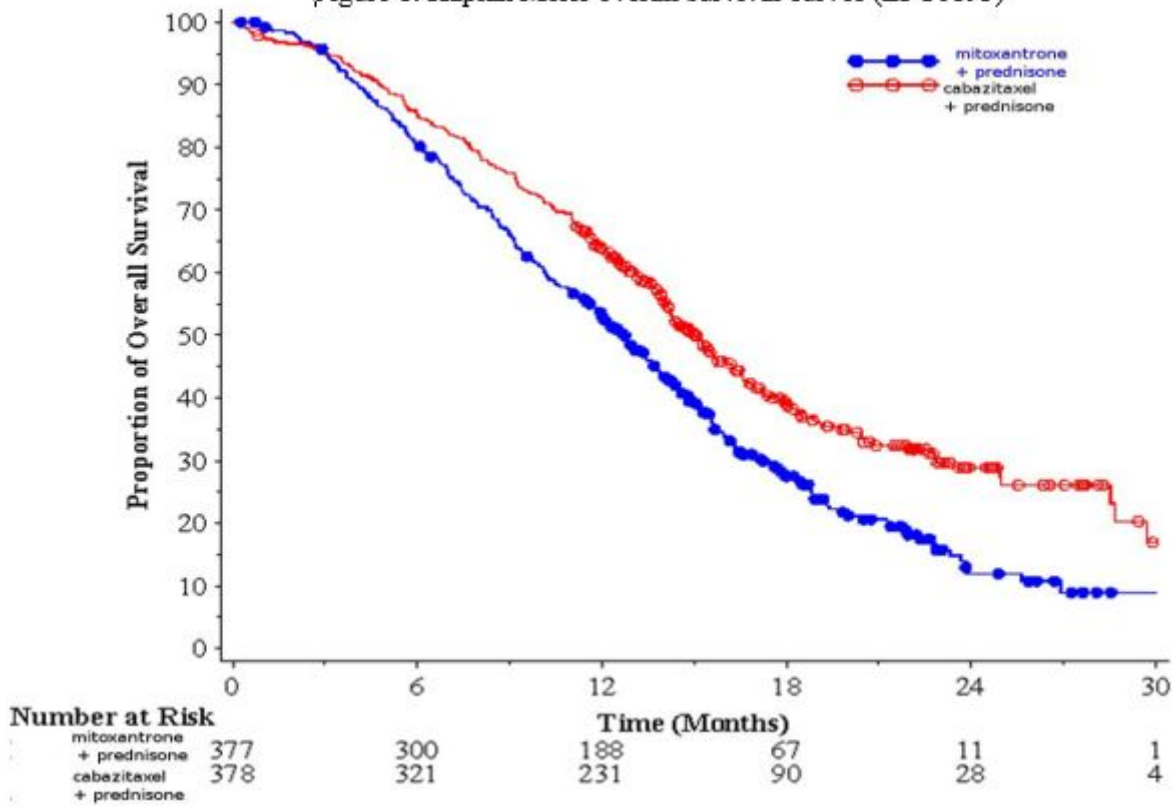
Figure 1: Kaplan Meier overall survival curves (EFC6193)
