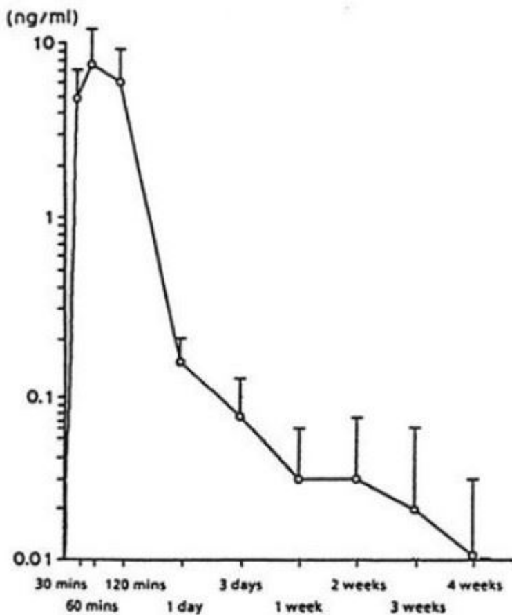
Figure 1: Leuporelin serum levels after single s.c. administration of 30 microgram/kg body weight of leuporelin acetate as Depot formulation (n=6) (Mean \pm SD)
